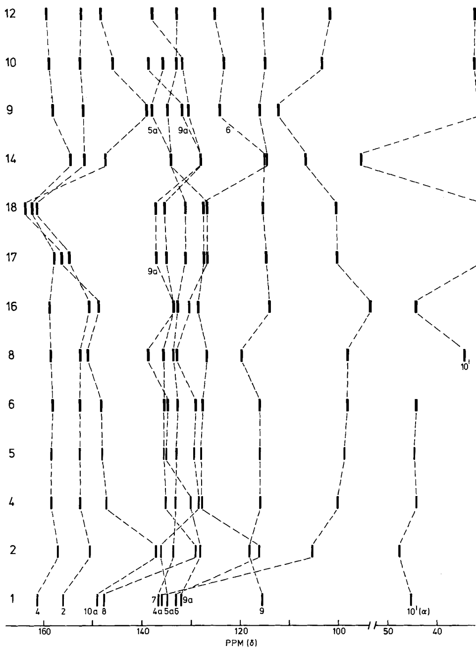
Fig. 3. ^{13}\text{C} -chemical shift correlation diagram for various flavin derivatives. The numbers on the horizontal axis refer to the C-atoms of the flavin molecule (cf. Scheme 1), the numbers on the vertical axis are related to the structure of the individual derivatives (cf. Scheme 2).
